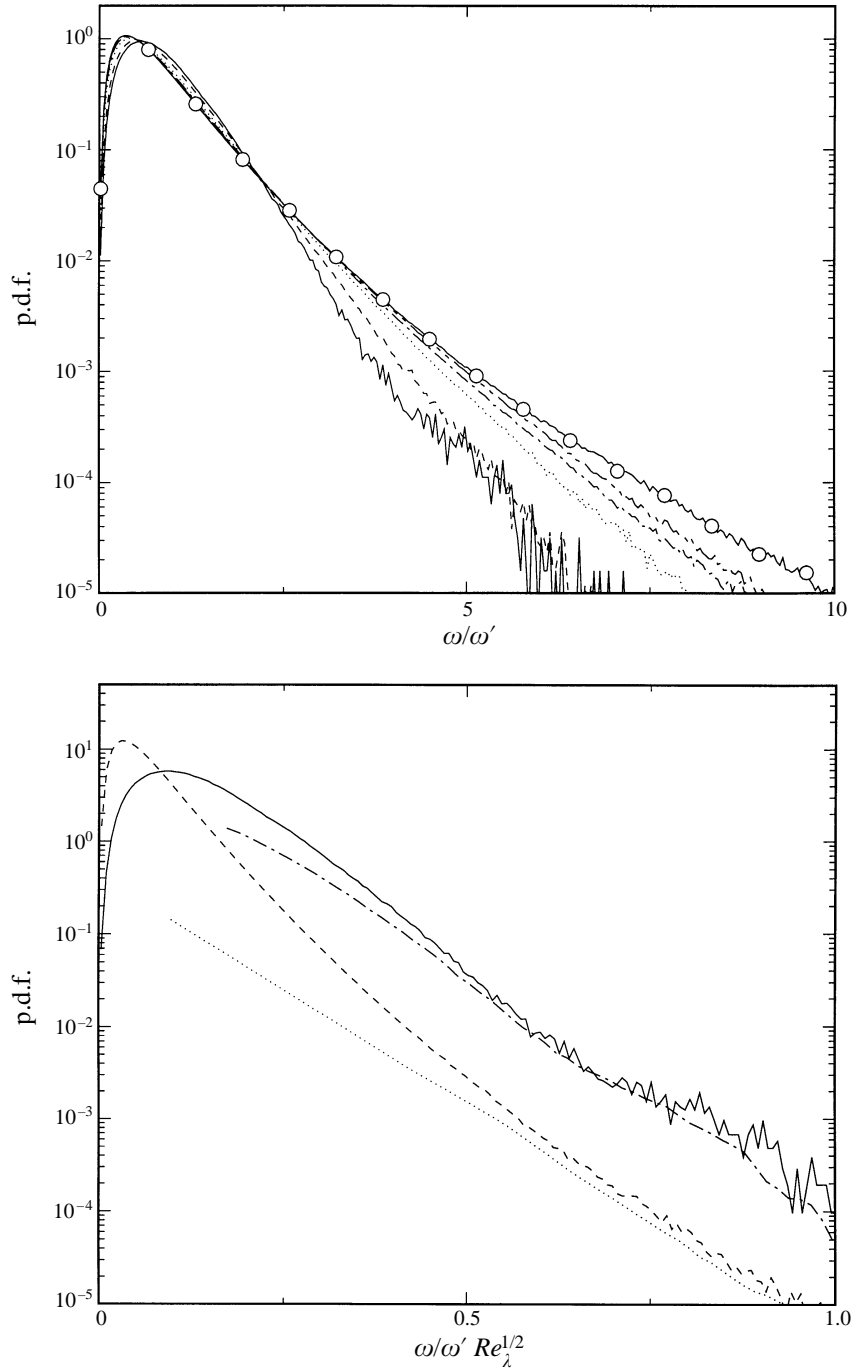
FIGURE 7. Probability density functions for the vorticity magnitude over the whole flow. (a) Calculated directly from the simulations in table 1. Lines as in table 1. (b) Tails of the p.d.f. for \omega > \omega' , computed from the filament statistics, compared to the actual distributions. Re_\lambda = 37 : —, from simulation; — · —, from filaments. Re_\lambda = 142 : - - - -, from simulation; ·····, from filaments.
